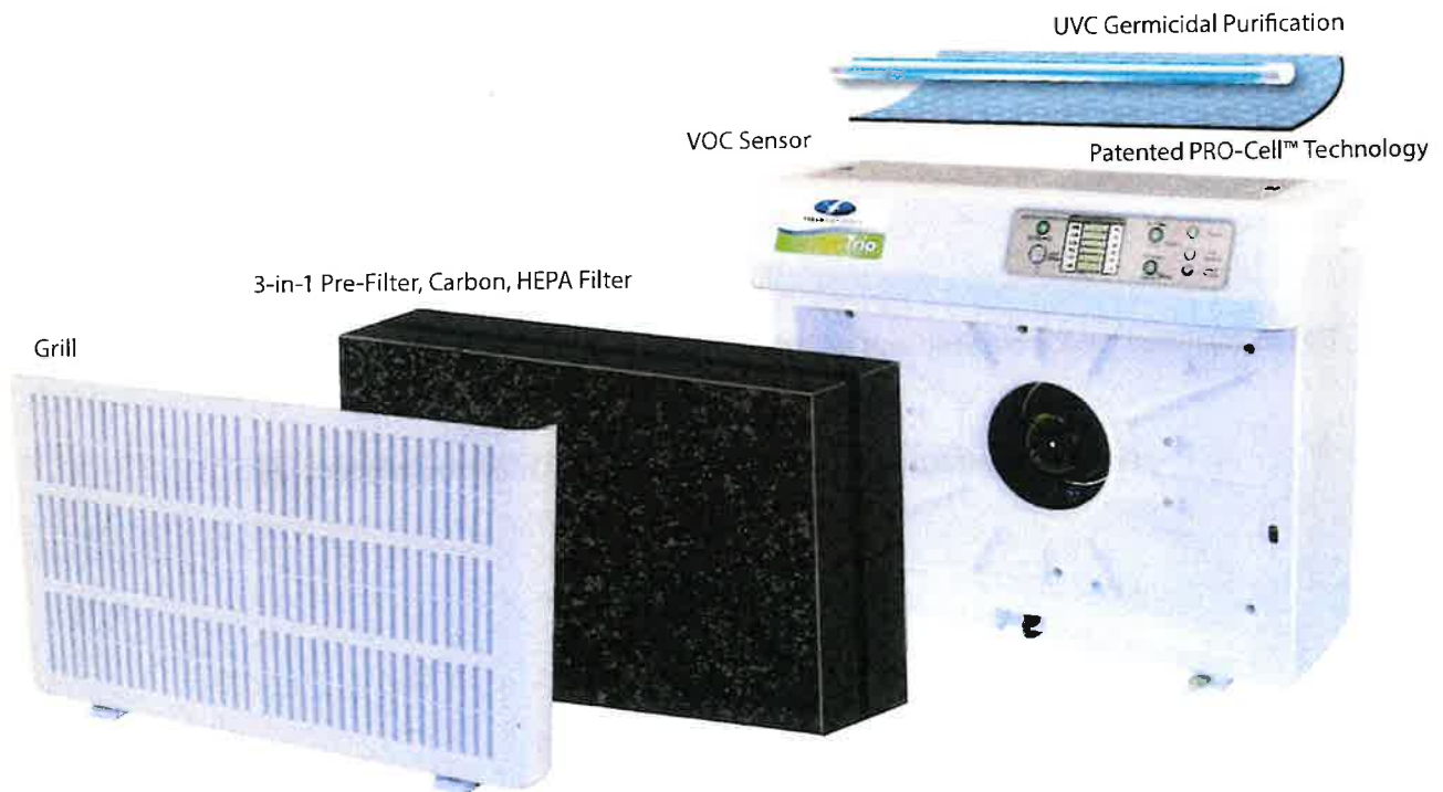
FIG 7 - STANDARD FILTER CONFIGURATION
