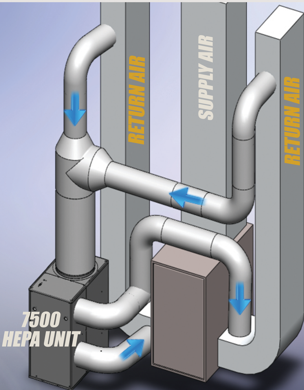
DUAL RETURN AIR SETUP, USING 7500 HEPA UNIT.
